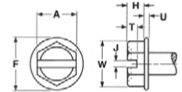
SLOTTED
